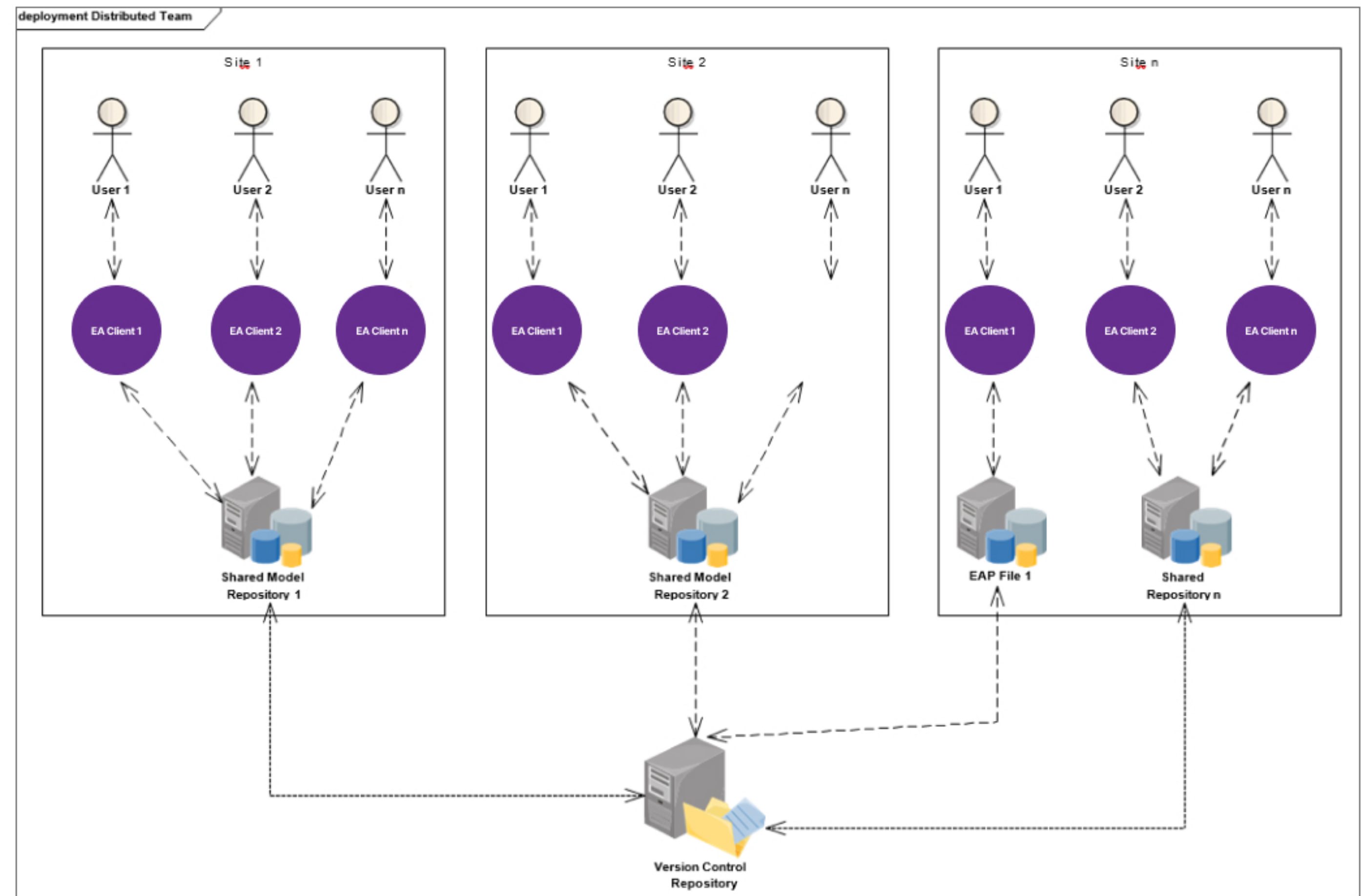
Figure 15: The Version Control Repository can facilitate replication of models across multiple development sites
