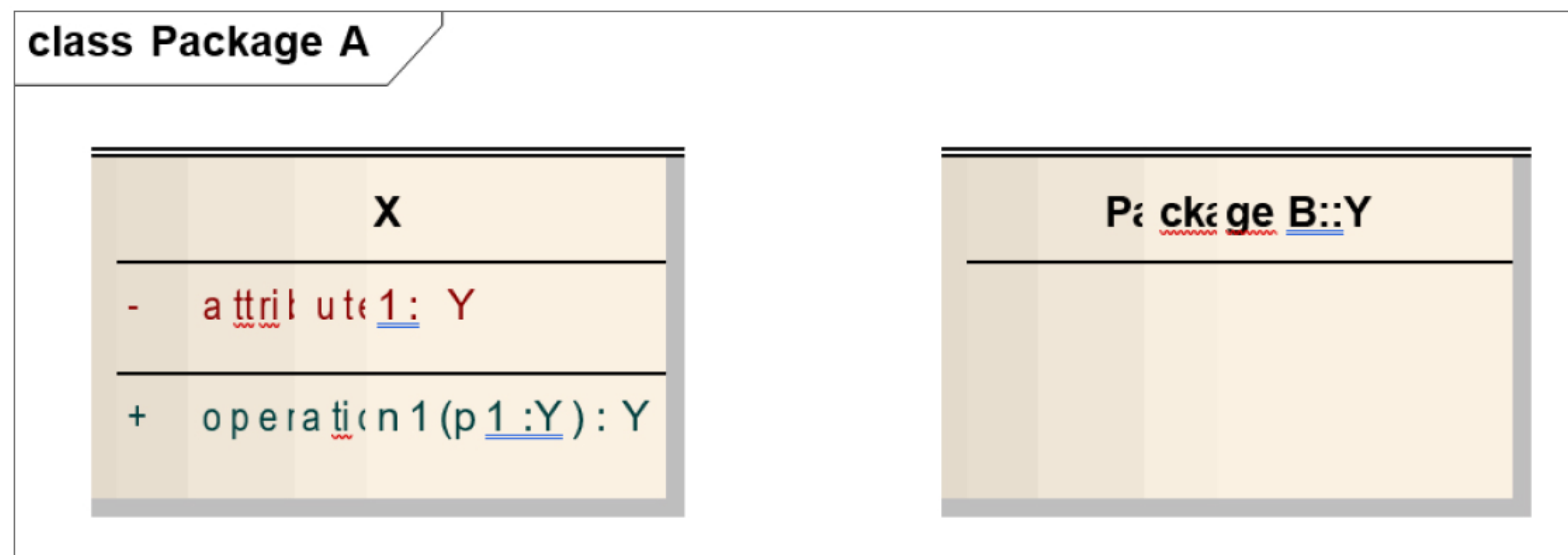
Figure 11: Class X refers to Class Y as a classifier for attribute and operation parameter types. Class Y is defined in a separately version controlled Package, Package B.
