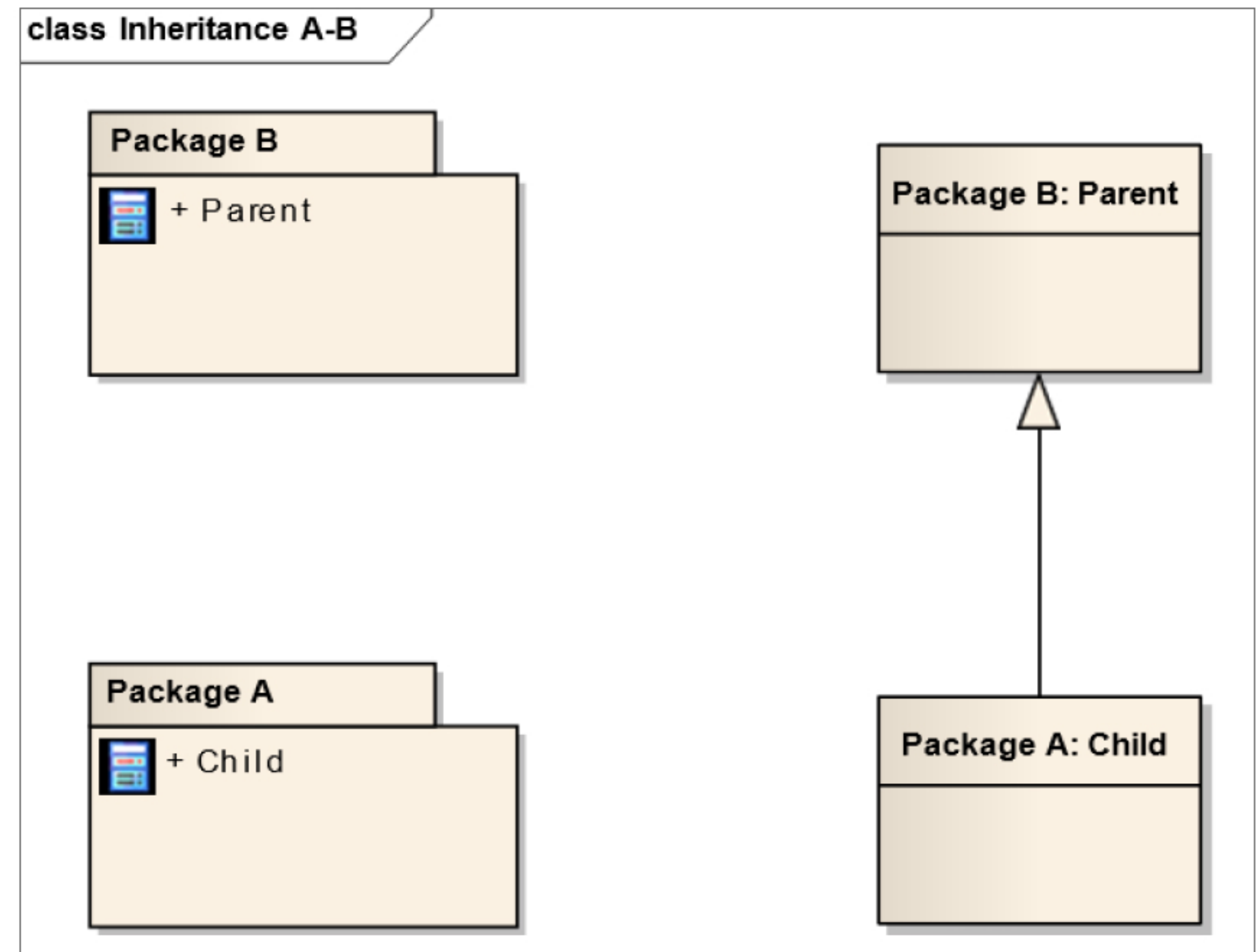
Figure 5: Parent and Child defined in separate Packages
