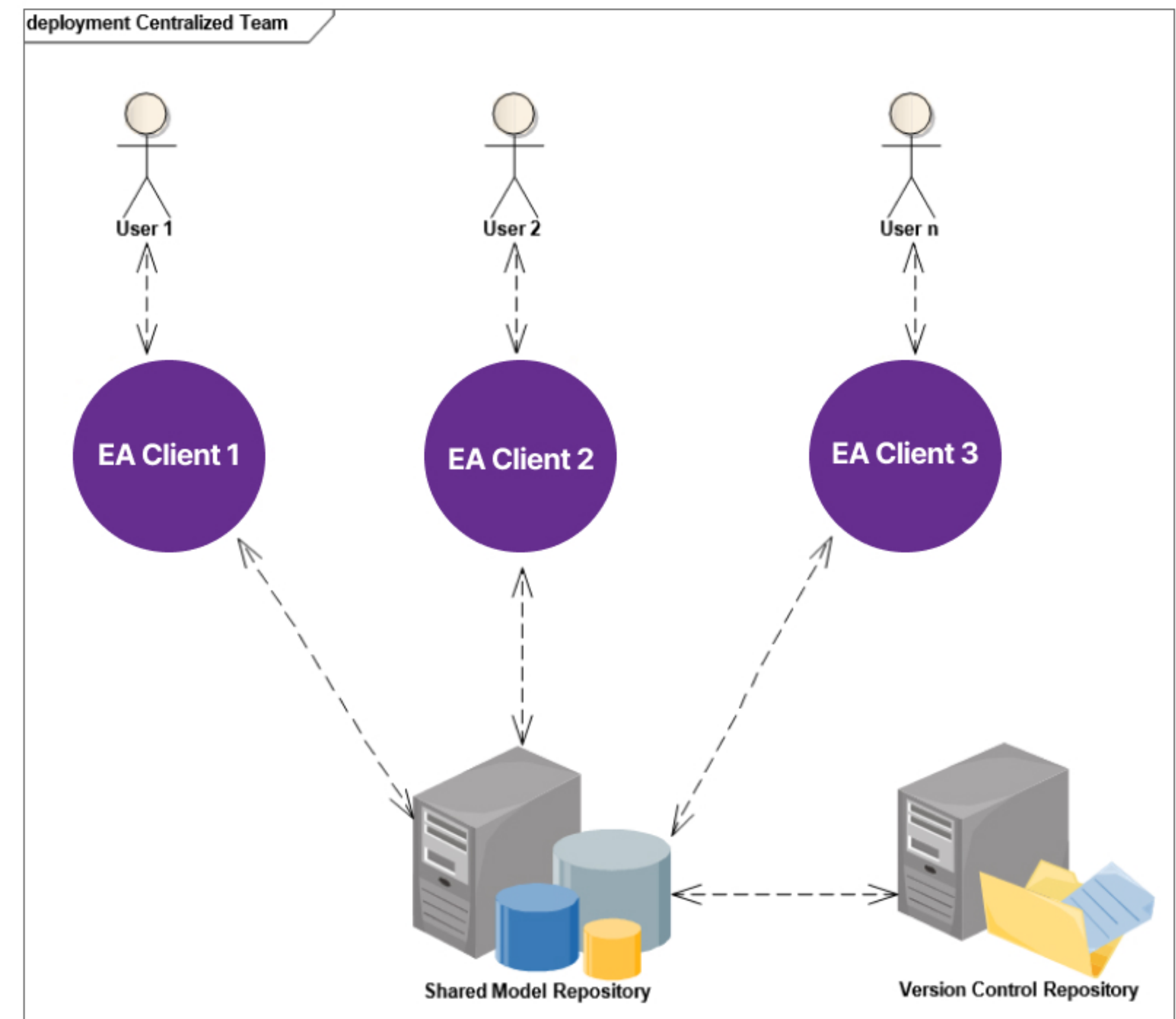
Figure 3: A Centralized Team connects to a common DBMS to edit the model
